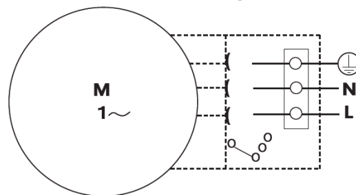
Electrical wiring
