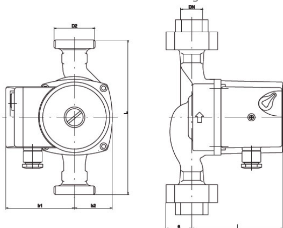
Dimension drawing
