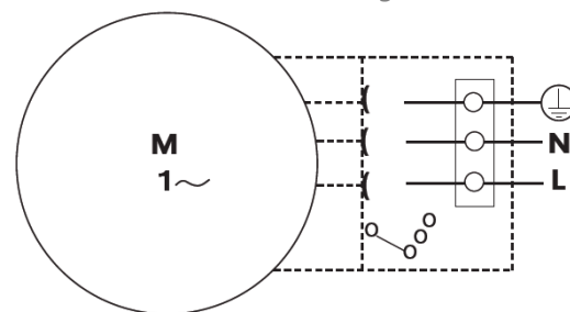
Electrical wiring
